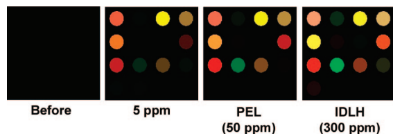
Figure 7. Difference maps of pigment-based arrays after 2 min \text{NH}_3 exposure. For purposes of display, the color range of these difference maps are expanded from 6 to 8 bits per color (i.e., RGB range of 4–67 expanded to 0–255). The full digital data and an HCA are provided in the Supporting Information, Table S2 and Figure S2.
